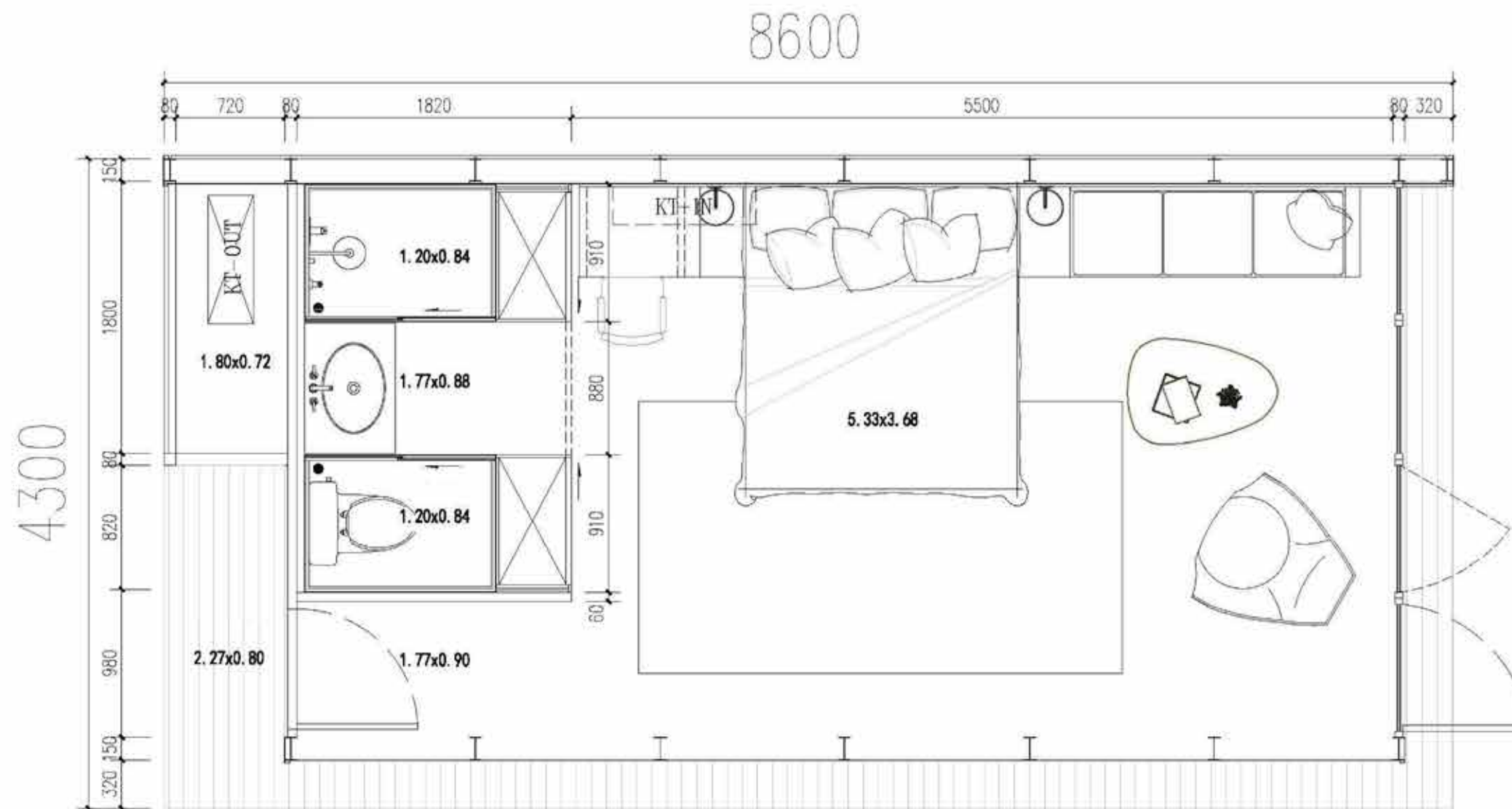
STANDARD FLOOR PLAN
